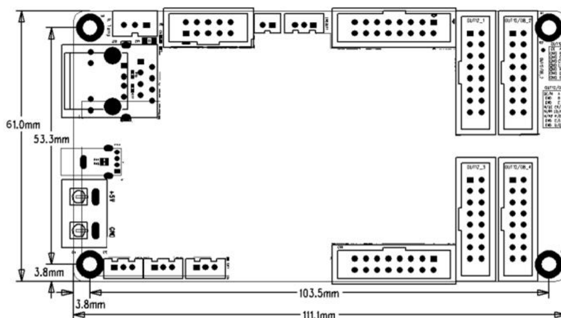
CPWB1S VER.B2 SILKSCREEN TOP
