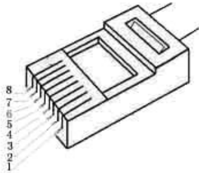
Figure 1 568B Network Cable Wiring Sequence
