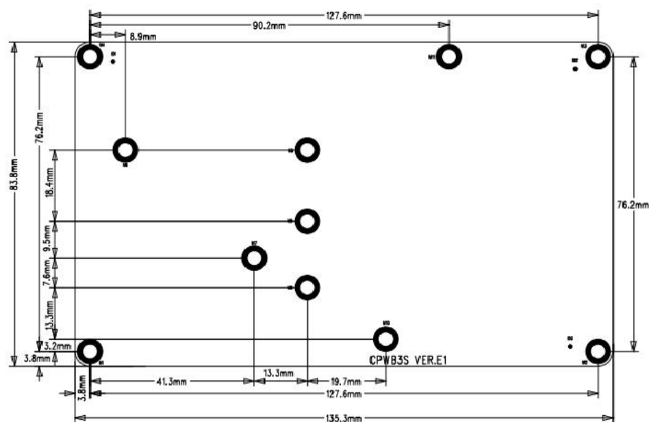
CPWB3S VER.E1 SILKSCREEN TOP
