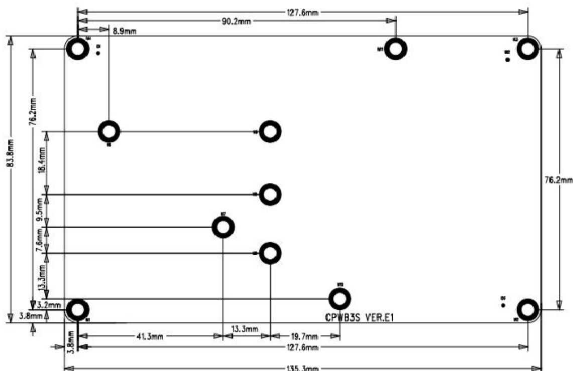
CPWB3S VER.E.1 SILKSCREEN TOP
