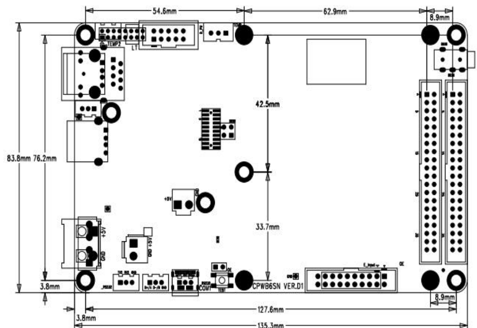
CPWB6SN VER.D1 SILKSCREEN TOP
