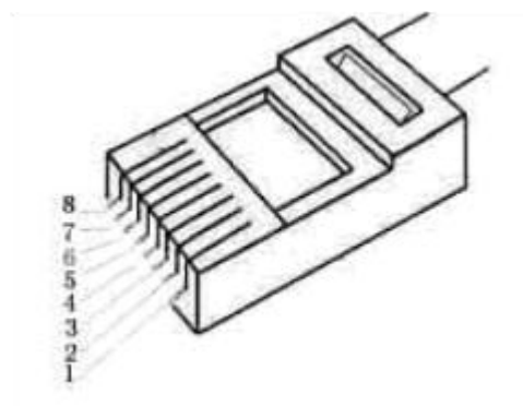
Figure 1 568B Network Cable Wiring Sequence
