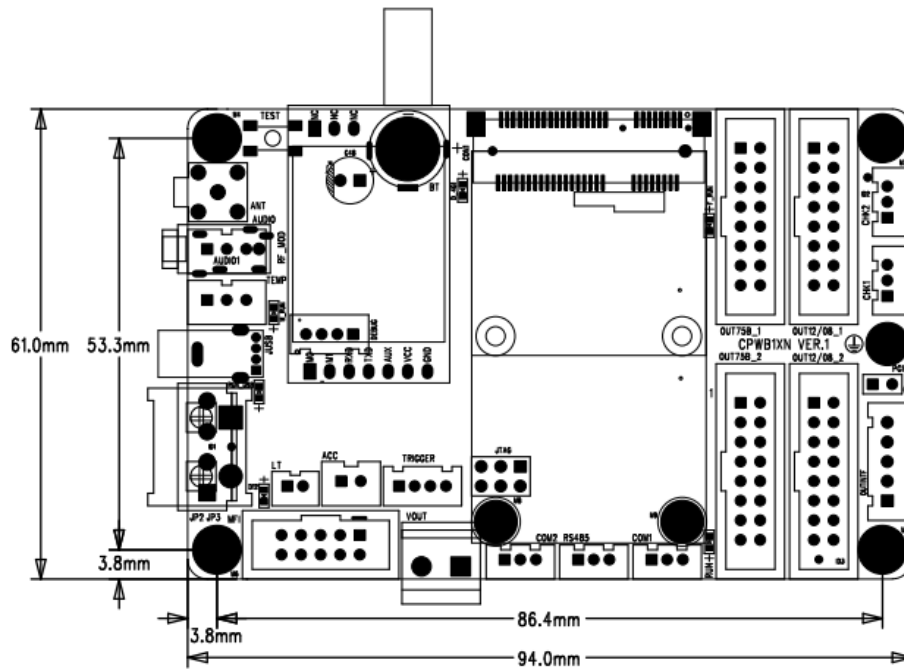
CPWB1XN VER.2 SILKSCREEN TOP
