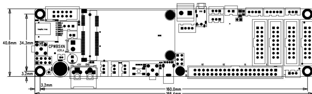
CPWB5XN VER.A SILKSCREEN TOP
